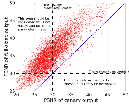
Figure 2: The PSNR of full-sized output versus the PSNR of canary output, for the I-frames of 106 videos on one of our application Boxblur-Vignette-Dilation video filter pipeline. The PSNR of full output is higher for over 98% approximation settings and 45.1% of the approximation settings lie in such a zone that is ignored by IRA approach but actually satisfies the quality requirement.
